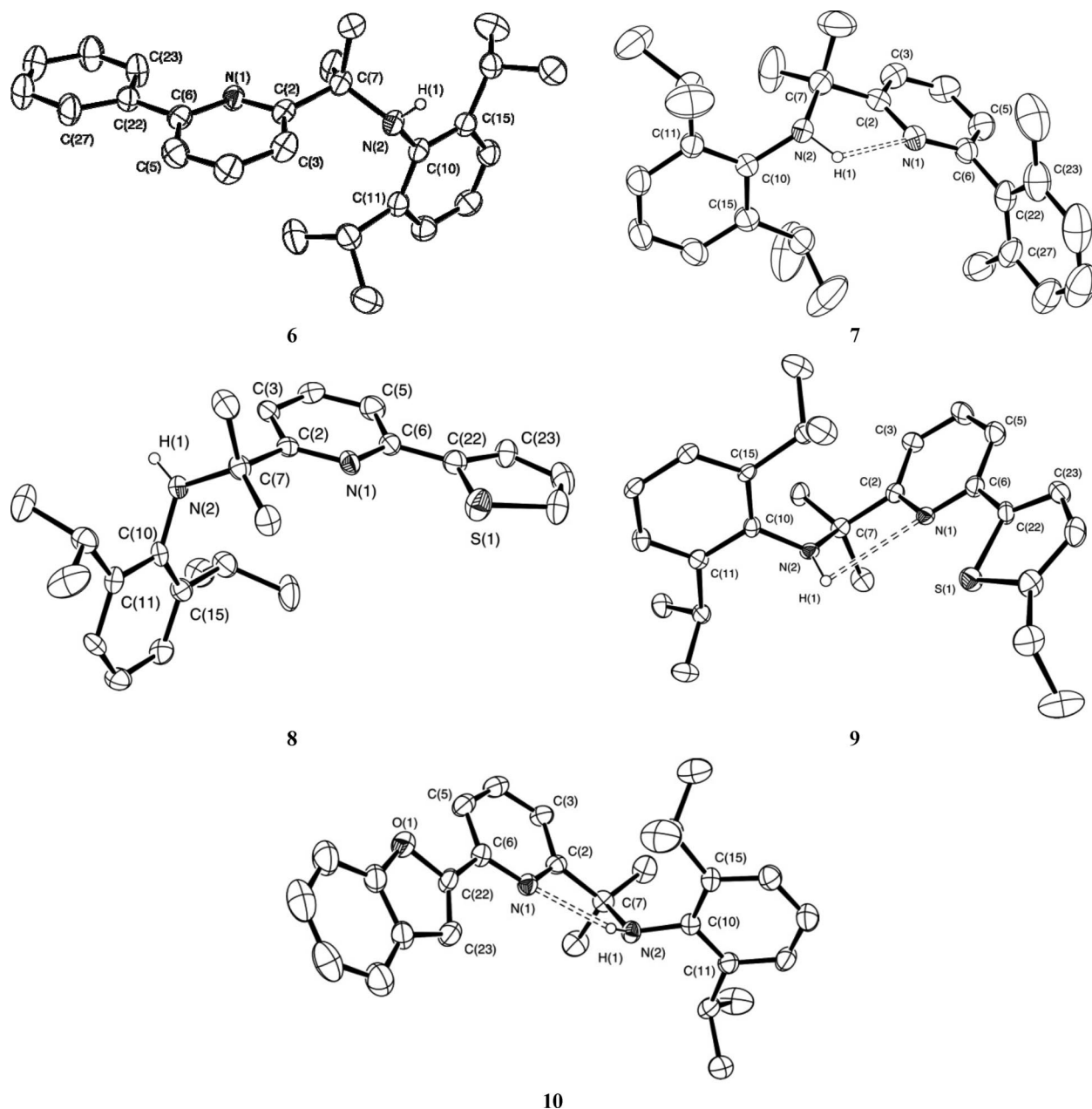
Figure 2. Crystal structures of ligands \text{N}_2\text{H}^{\text{Ph}} ( 6 ), \text{N}_2\text{H}^{\text{Xyl}} ( 7 ), \text{N}_2\text{H}^{\text{Th}} ( 8 ), \text{N}_2\text{H}^{\text{EtTh}} ( 9 ) and \text{N}_2\text{H}^{\text{BFu}} ( 10 ). Thermal ellipsoids are drawn at the 30% probability level. Hydrogen atoms, apart from those of the N–H moiety, are omitted for clarity.
