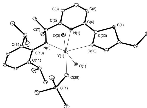
Figure 4. Crystal structure of [N_2^{EtTh}Y(CH_2SiMe_3)(thf)_2] ( 14 ). Thermal ellipsoids are drawn at the 30% probability level. Hydrogen atoms and methylene groups of the thf molecules are omitted for clarity.
